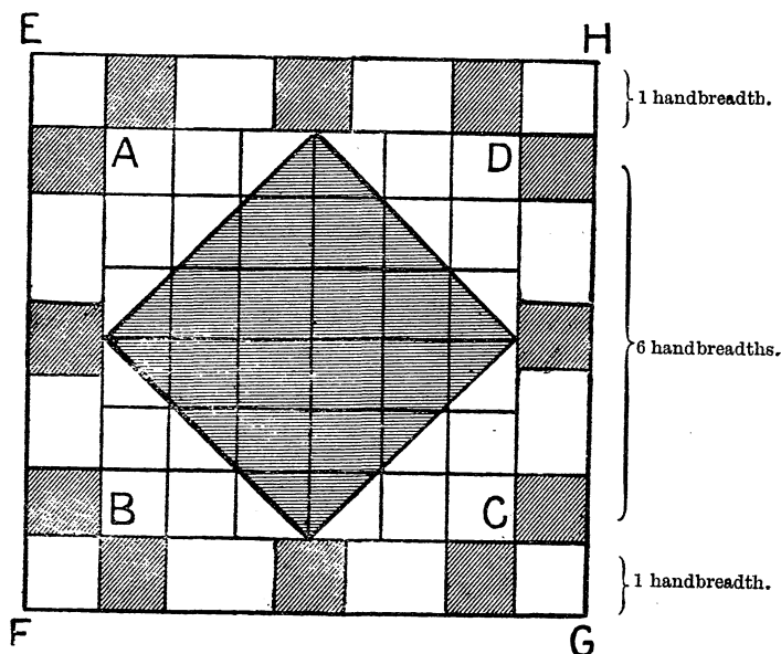
FIG. 15.—PROBLEM ON MAXIMA AND MINIMA (CASE II).
